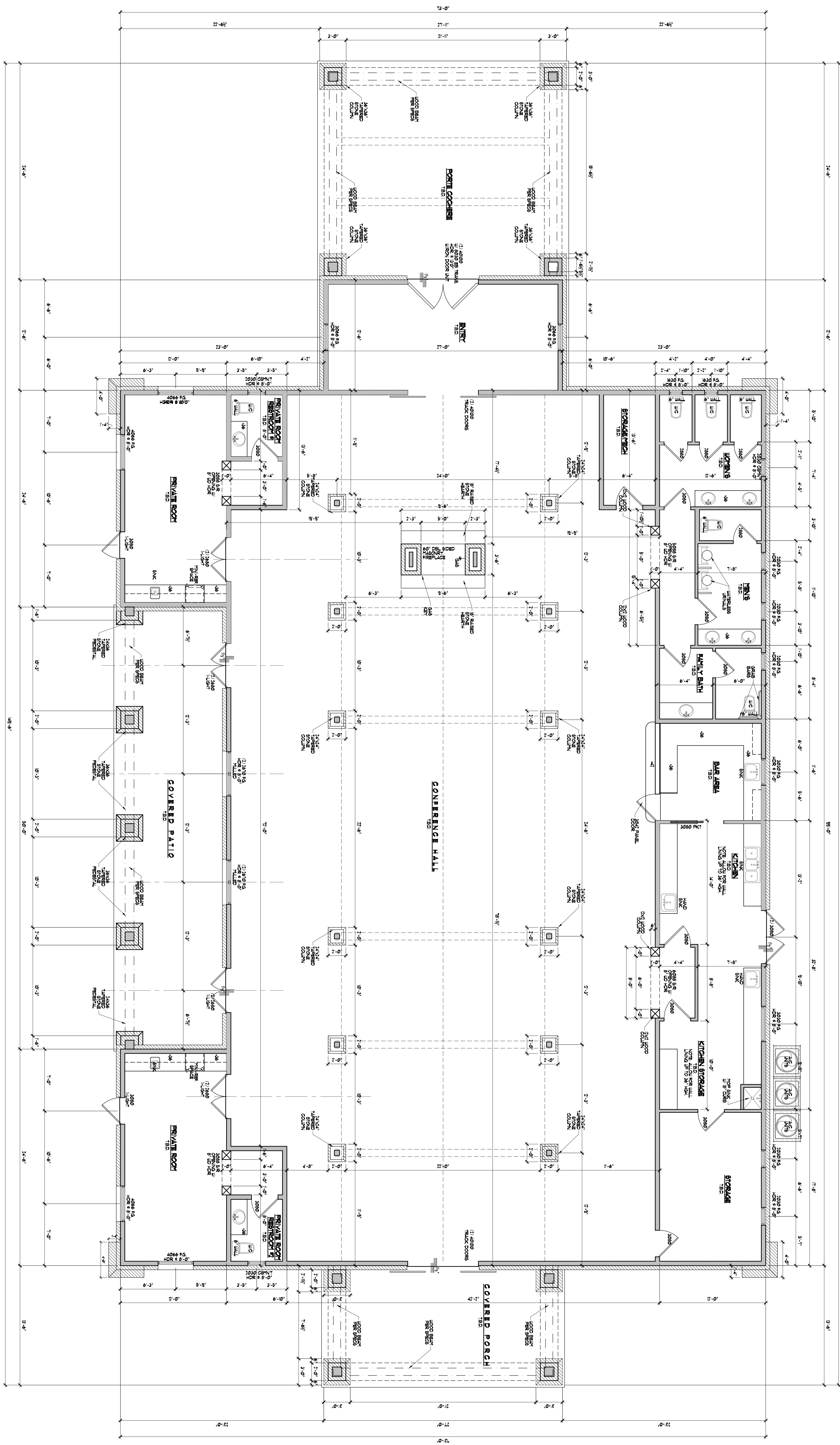
FLOOR PLAN SCALE: 1/4" = 1'-0"
